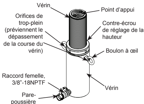
Figure 1 - Composants de vérin type
