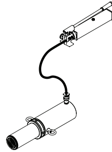
Figure 2 - Illustration to bleed air from system
