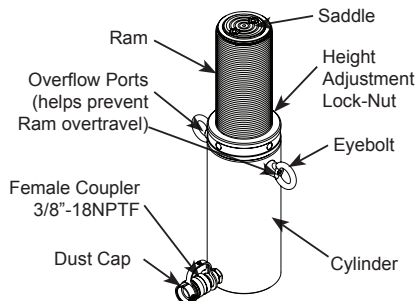
Figure 1 - Typical Cylinder Components
