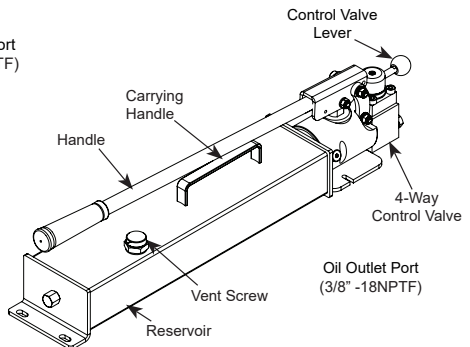
Figure 2 - Model P2601M Components
