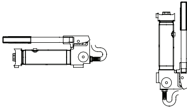
Figure 5 - Horizontal and Vertical Position
