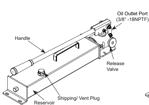
Figure 1 - Model P2601 Components
