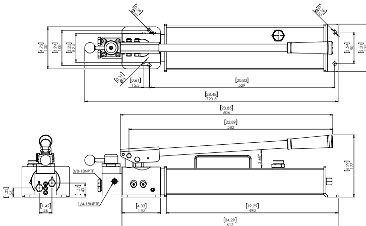
Figure 4 - P2601M Dimensions
