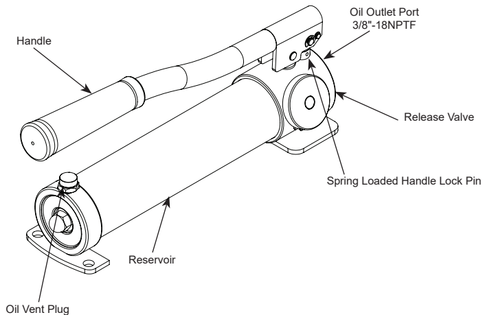
Figure 1 - Components
